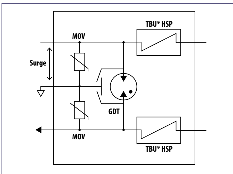
Figure 7. | Hybrid Primary and Secondary Protector
