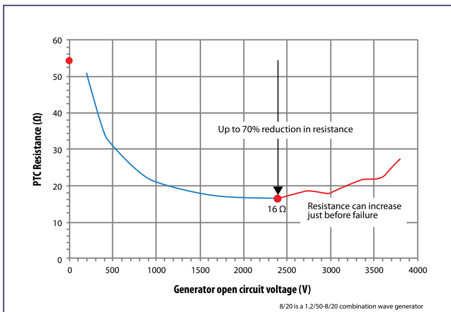
Figure 5. | CMF-RL55-0-A1 Resistance During 8/20 \mu s Generator Resistance = 2 \Omega
