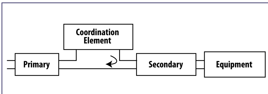
Figure 2. | Current-Type Coordination
